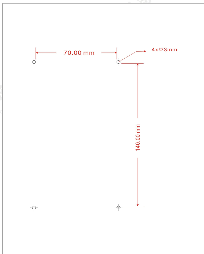
FY100—Hole installation drawing
