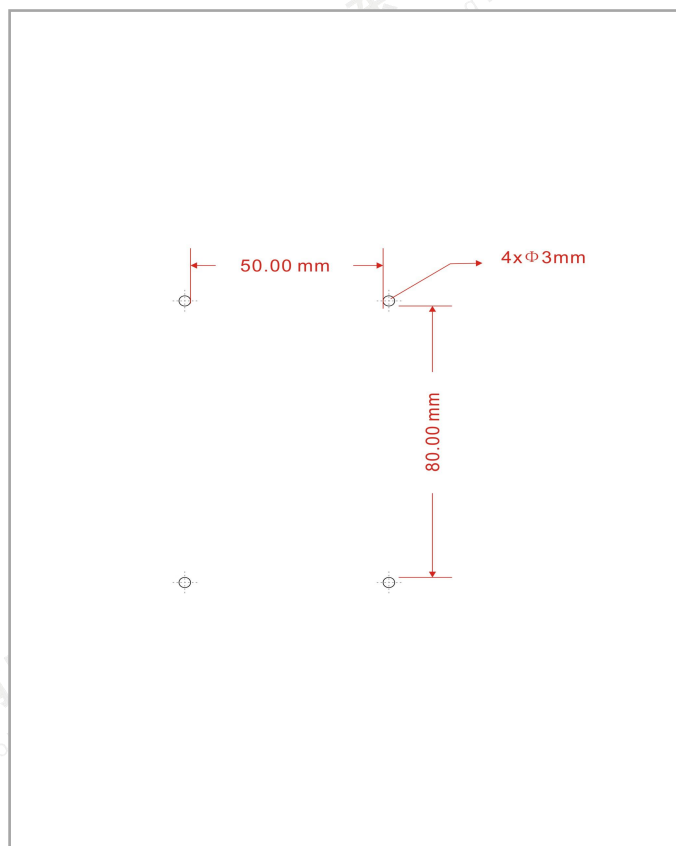
FY200—Hole installation drawing
